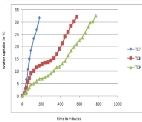
Figure 14. Effect of Ethylcellulose coating level on % water uptake of time controlled Release tablets with 10 mg/ cm 2 Ac-Di-Sol layer
